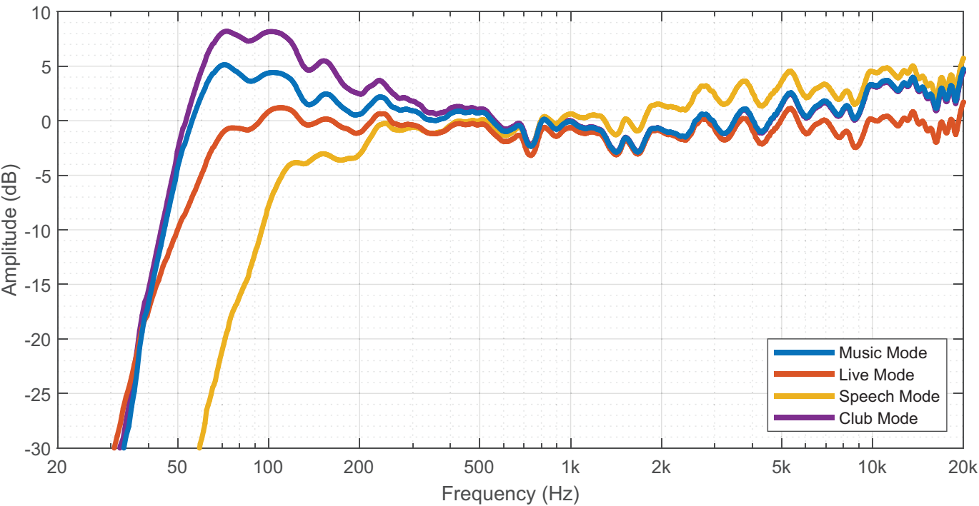
Fig. 2: Frequency response
